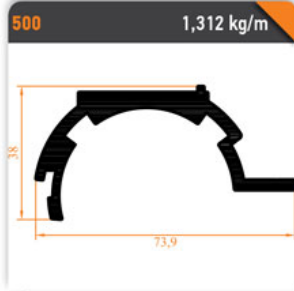
Kelepçe Clamp
